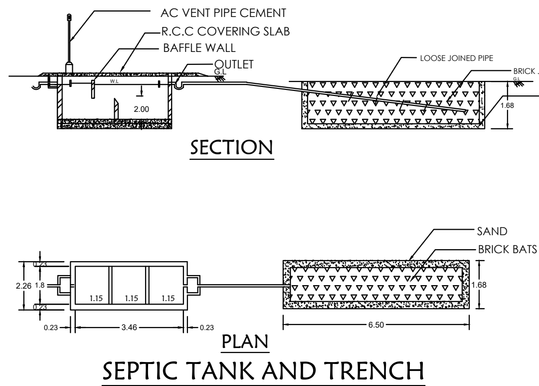
PLAN SEPTIC TANK AND TRENCH
