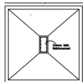
COLUMN FOUNDATION DETAIL PLAN OF FOOTING
