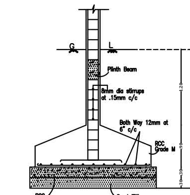
SECTION OF FOOTING
