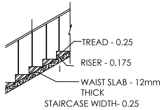
STAIR CASE DETAIL
