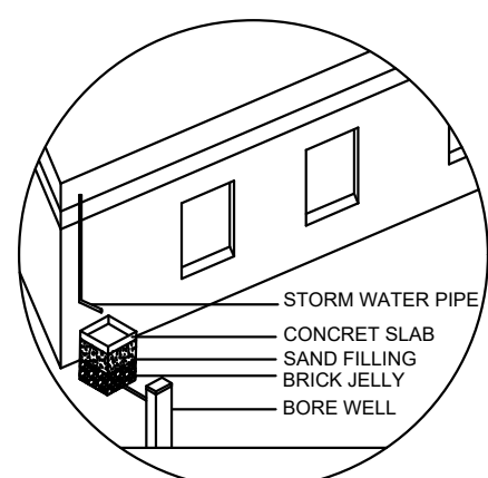
DETAIL RAINWATER HARVESTING
