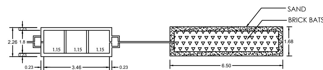
PLAN SEPTIC TANK AND TRENCH
