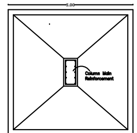
COLUMN FOUNDATION DETAIL PLAN OF FOOTING
