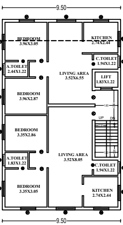
THIRD FLOOR PLAN
