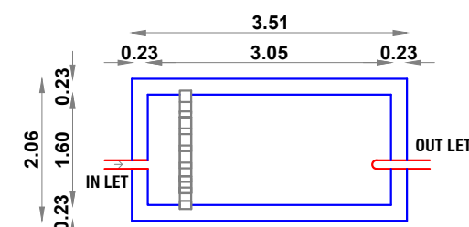
PLAN OF SEPTIC TANK CAPACITY - 8000 LITRES
