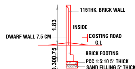
SECTION OF COMPOUND WALL
