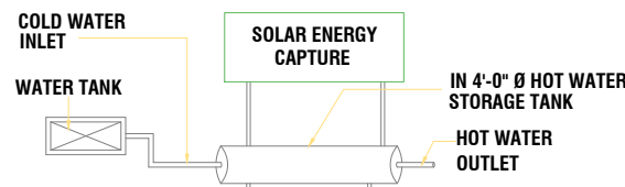
SOLAR HOT WATER SYSTEM DETAIL
