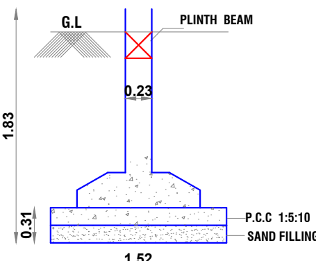
FOUNDATION DETAIL
