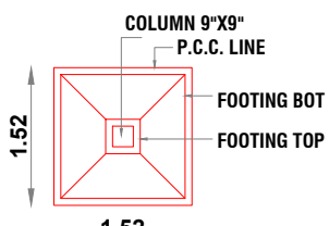
PLAN OF FOOTING
