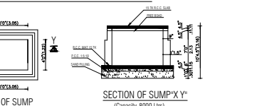
SECTION OF SUMP "X-Y"
