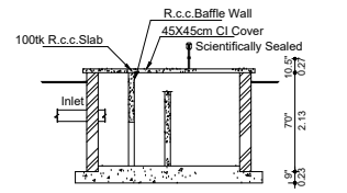
SECTION OF SEPTIC TANK "X-Y"
