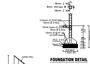
FOUNDATION DETAIL
