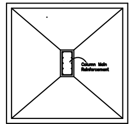
COLUMN FOUNDATION DETAIL PLAN OF FOOTING
