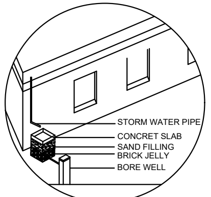
DETAIL RAINWATER HARVESTING
