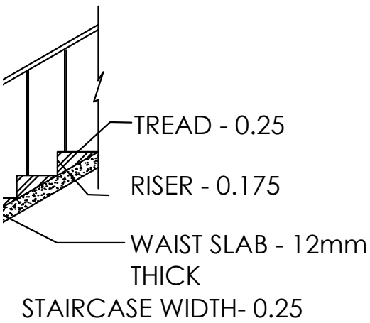
CASE DETAIL
