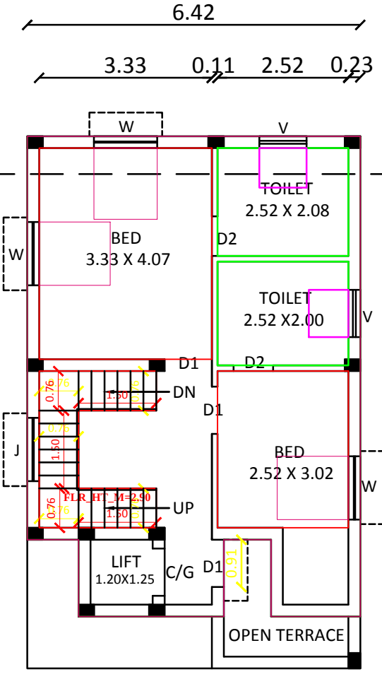
PRO. SECOND FLOOR PLAN
