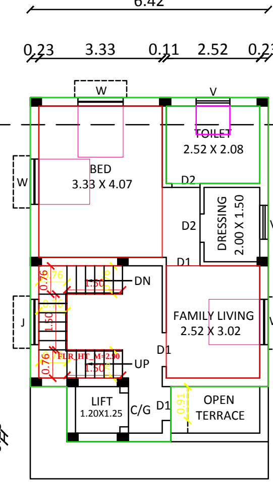
PRO. THIRD FLOOR PLAN
