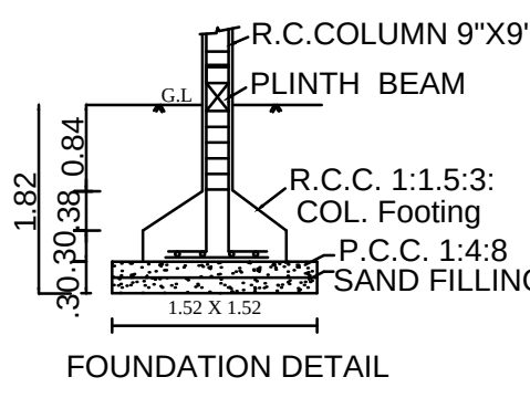
FOUNDATION DETAIL
