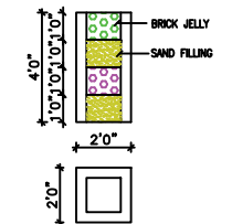
PERCOLATION PIT
