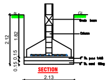
SECTION 2-13
