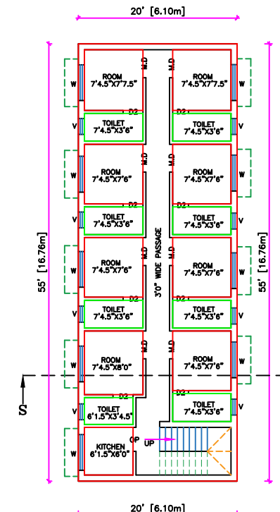
PRO. THIRD FLOOR PLAN
