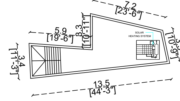
PROPOSED TERRACE FLOOR
