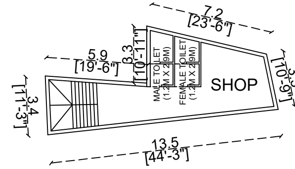
PROPOSED SECOND FLOOR COMMERCIAL PLAN
