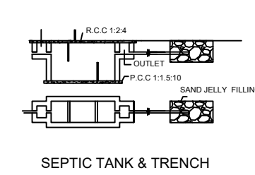
SEPTIC TANK & TRENCH (Not to scale)
