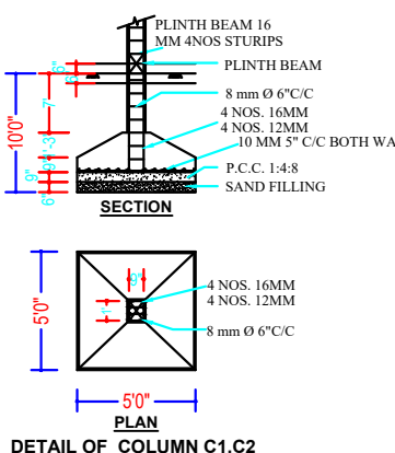
DETAIL OF COLUMN C1,C2
