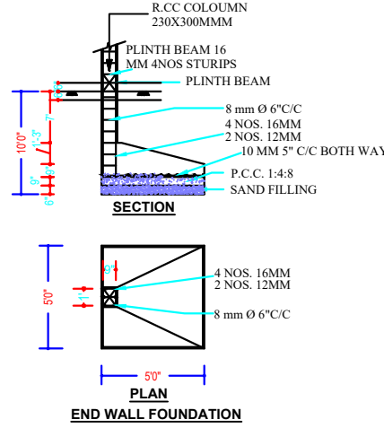
END WALL FOUNDATION
