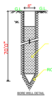
BORE WELL DETAIL
