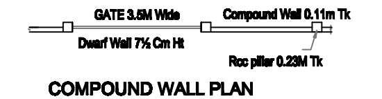
COMPOUND WALL PLAN
