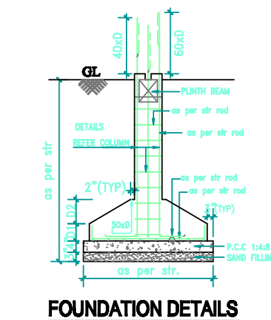
FOUNDATION DETAILS
