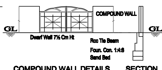
COMPOUND WALL DETAILS SECTION
