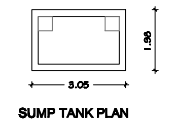
SUMP TANK PLAN
