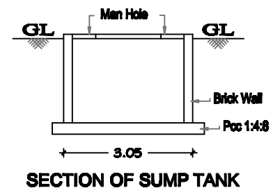
SECTION OF SUMP TANK
