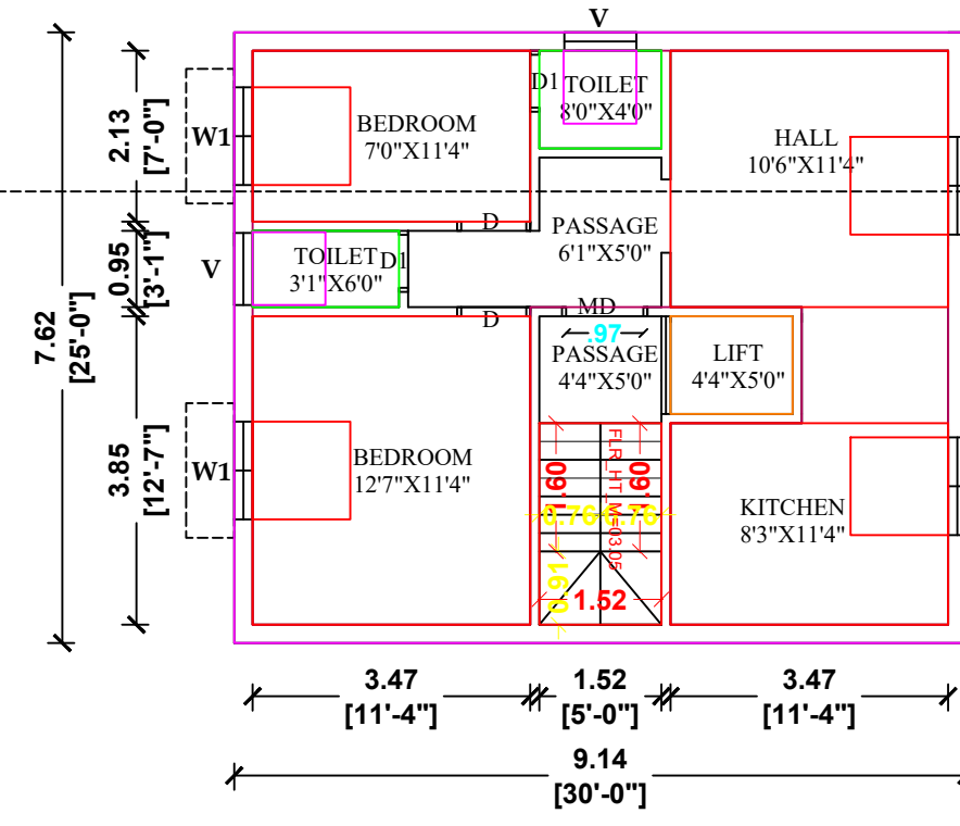
PROPOSED THIRD FLOOR PLAN
