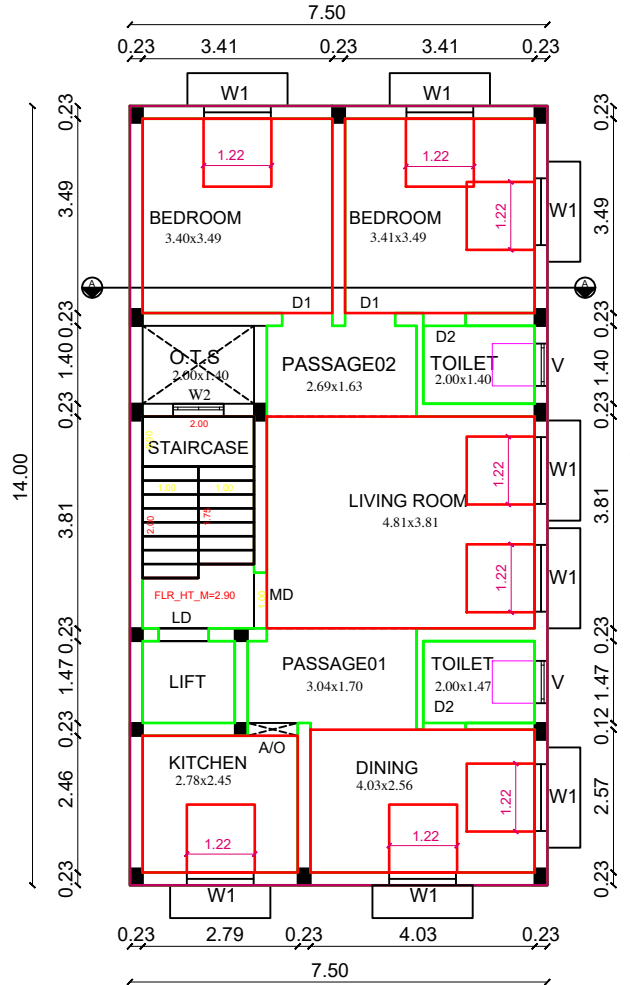
SECOND FLOOR PLAN (PROPOSED)
