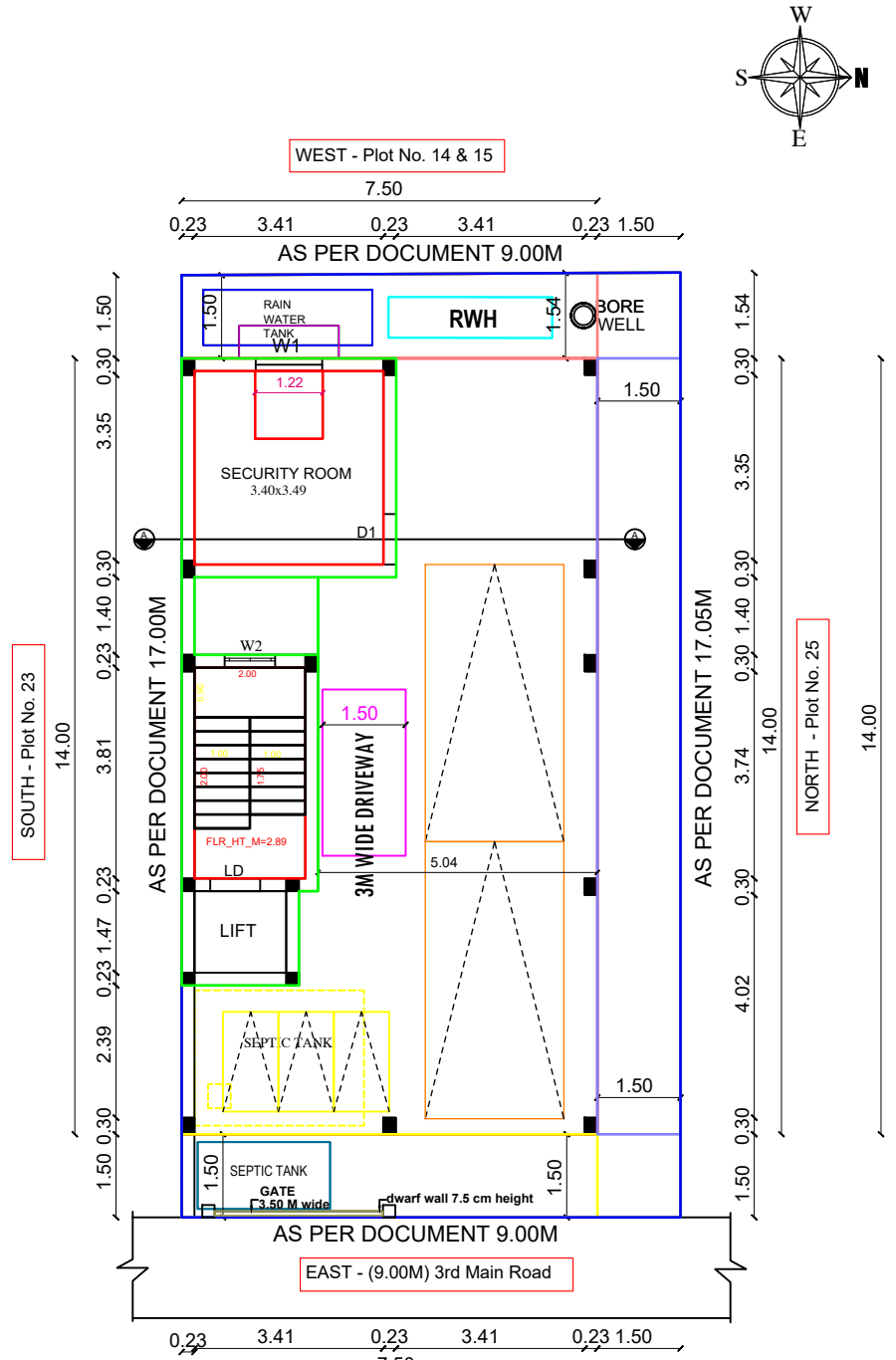
QR PLAN
