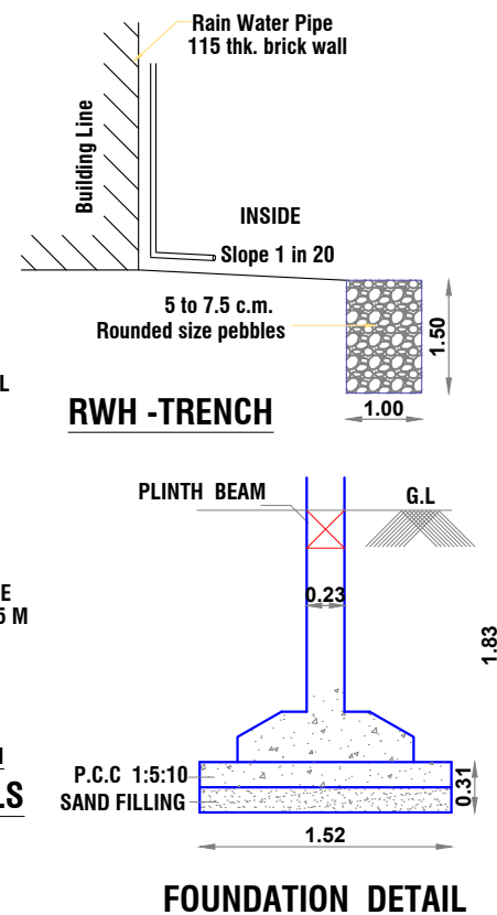
FOUNDATION DETAIL
