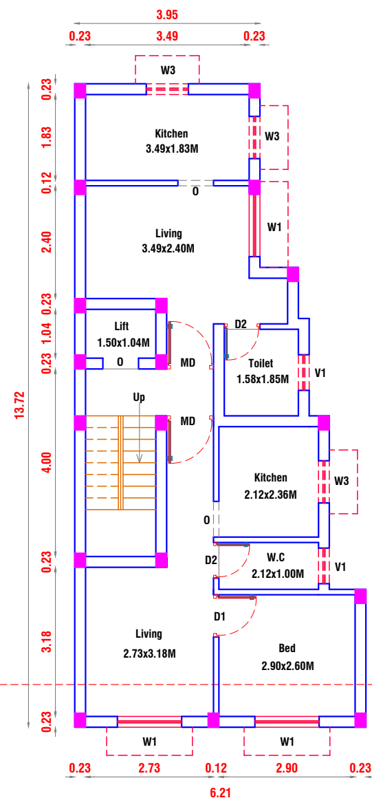
THIRD FLOOR PLAN
