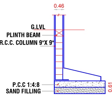
END FOOTING DETAILS
