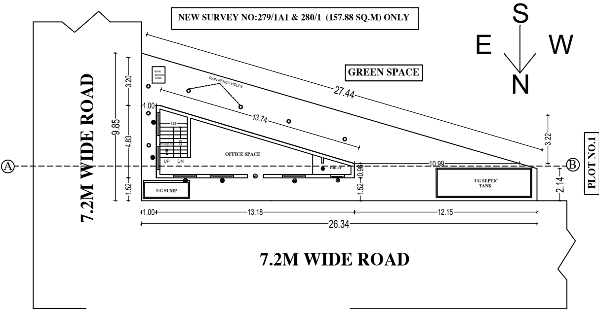
FLOOR PLAN
