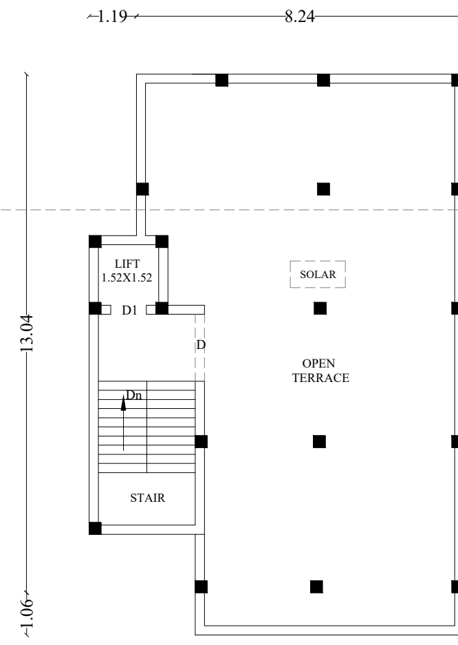
TERRACE FLOOR
