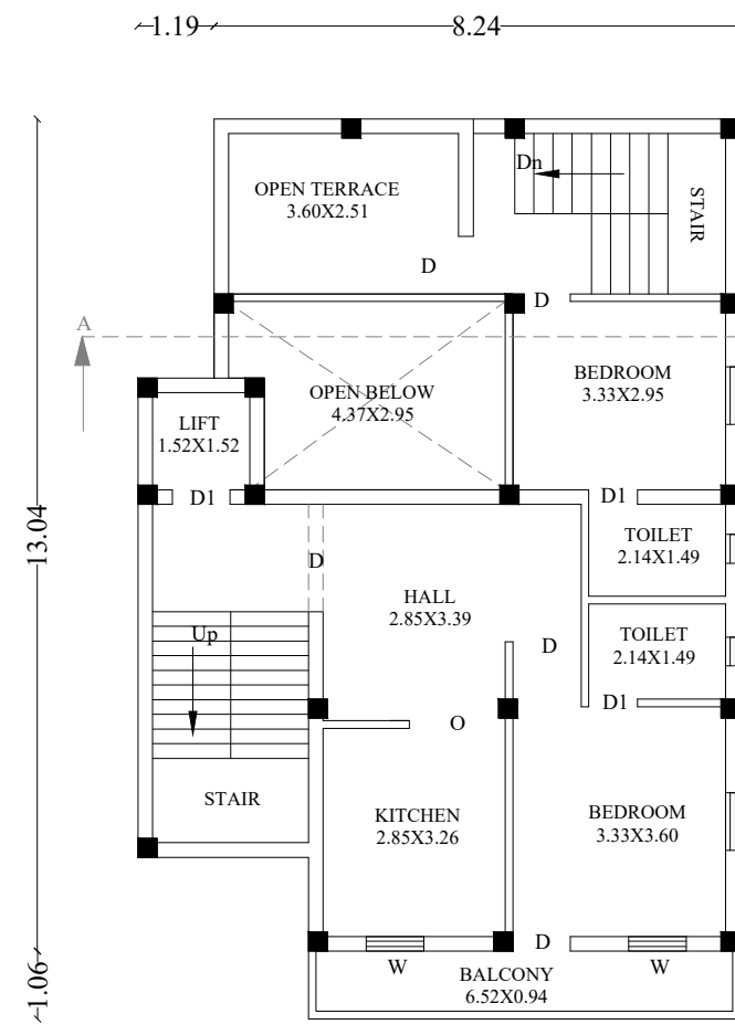
THIRD FLOOR
