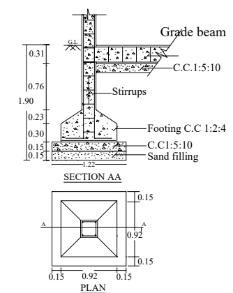
FOUNDATION DETAILS
