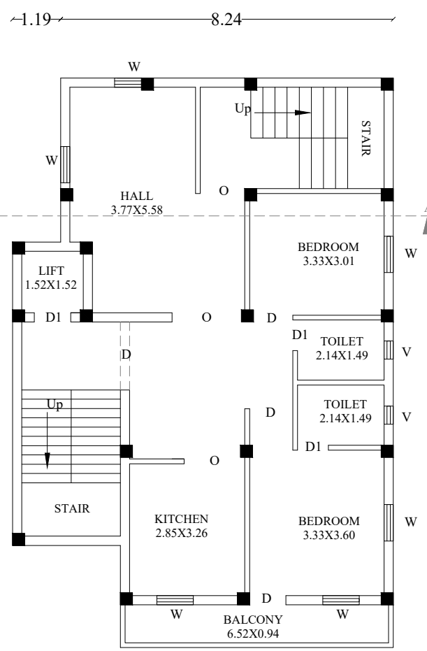
SECOND FLOOR
