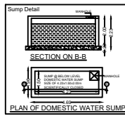
PLAN OF DOMESTIC WATER SUMP
