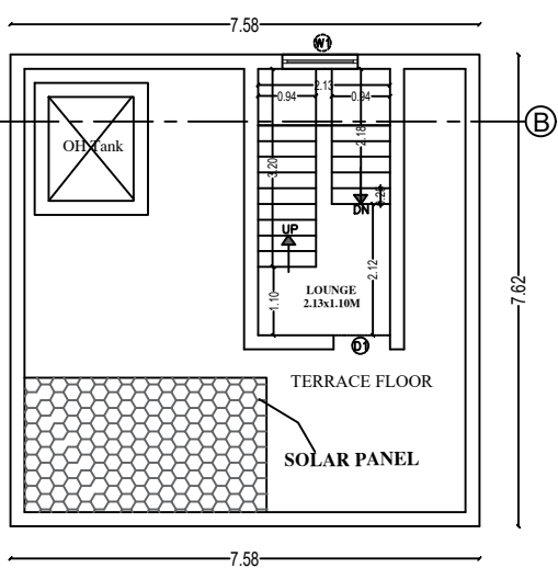
PROPOSED TERRACE FLOOR PLAN
