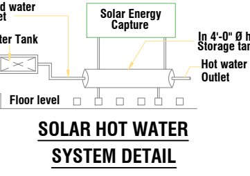
PERCUSSION PIT
