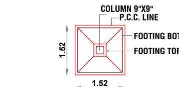
PLAN OF FOOTING
