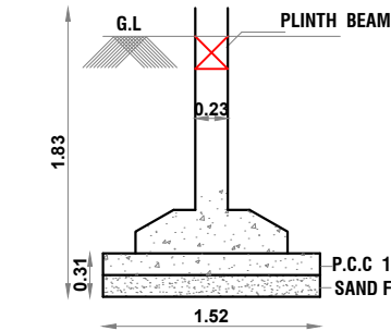
FOUNDATION DETAIL
