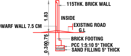
SECTION OF COMPOUND WALL
