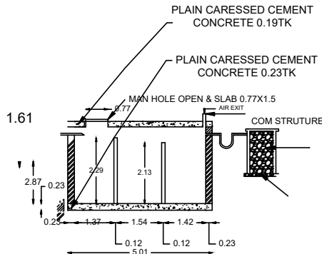
SECTION XX
