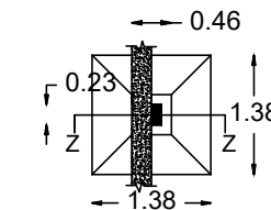
COLUMN FOOTING DETAIL
