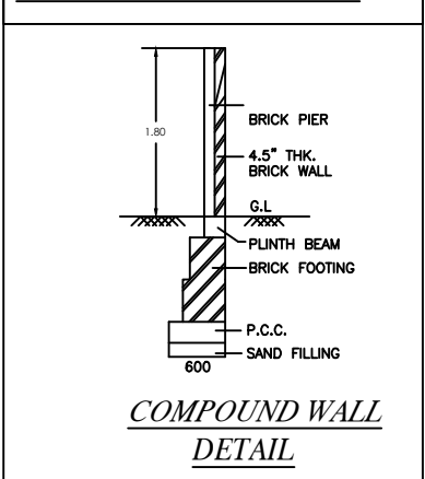
COMPOUND WALL
