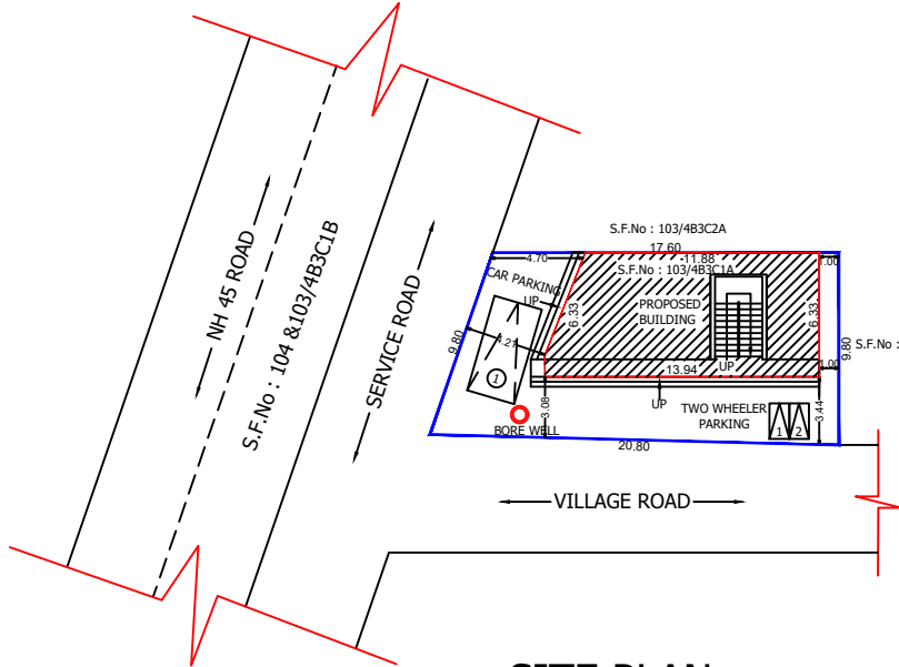
SITE PLAN
