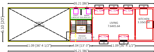
THIRD FLOOR
