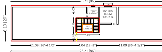
STILT FLOOR
