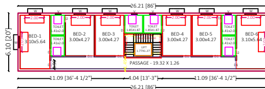
FIRST FLOOR
