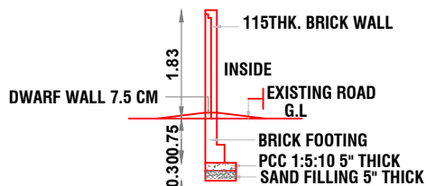
SECTION OF COMPOUND WALL
