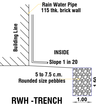
RWHTRENCH
