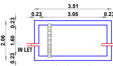
PLAN OF SEPTIC TANK CAPACITY - 8000 LITRES
