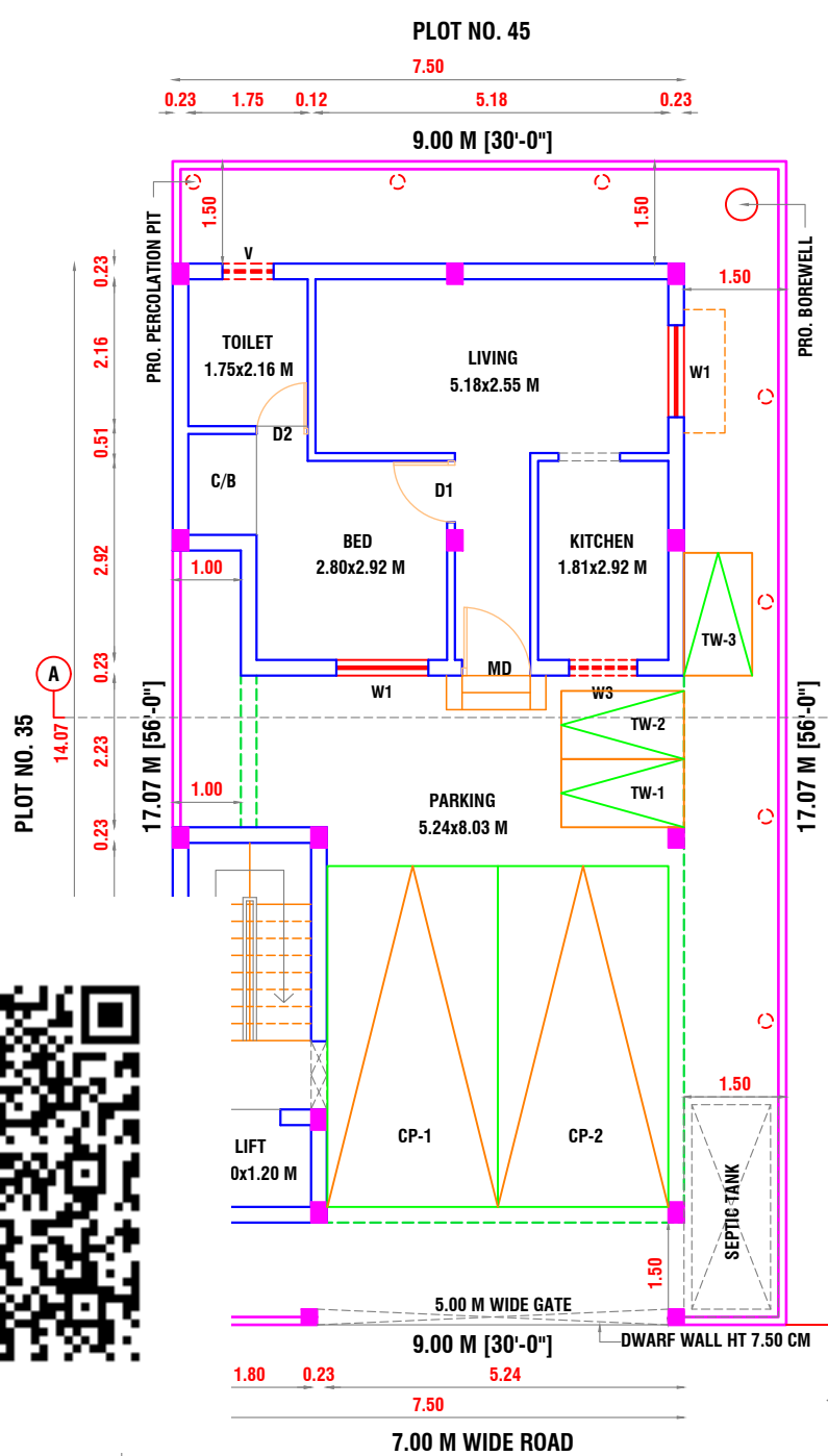
SITE CUM GROUND FLOOR PLAN
