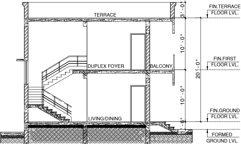
SECTION - XX
