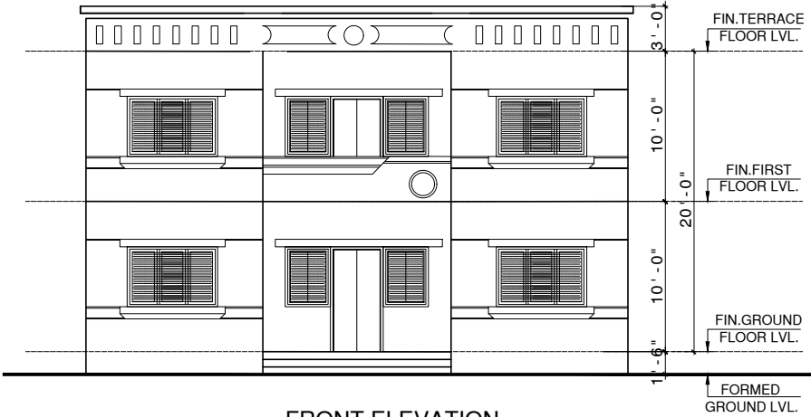
FRONT ELEVATION
