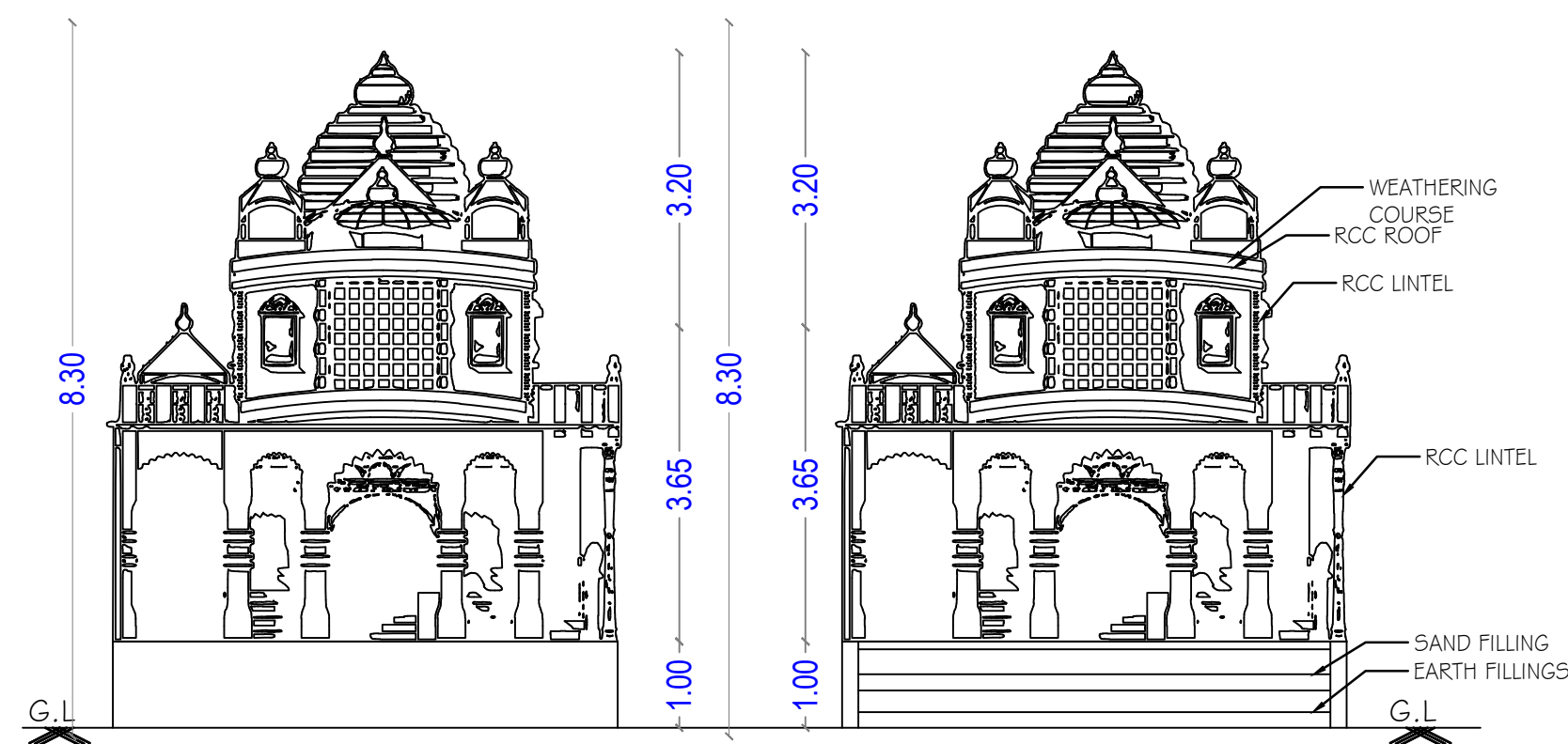
ELEVATION (PROPOSED)
