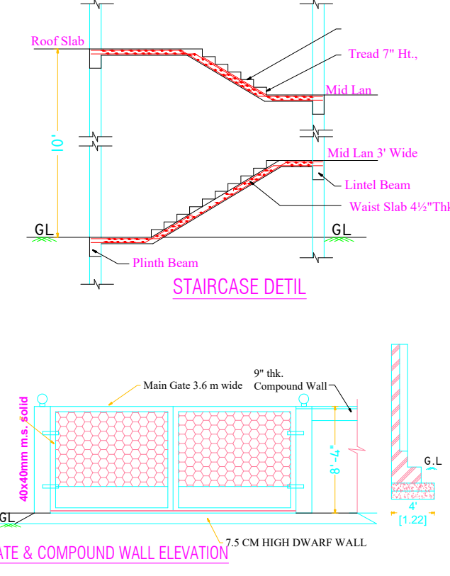
STAIRCASE DETAIL
