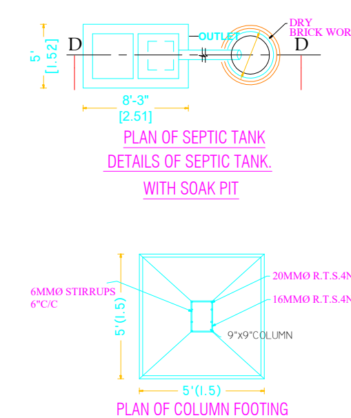
PLAN OF SEPTIC TANK WITH SOAK PIT
