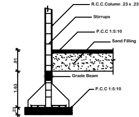
COLUMN DETAIL
