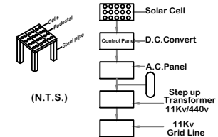
SOLAR SYSTEM FLOW DIAGRAM
