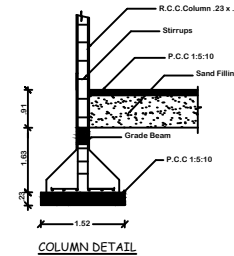
COLUMN DETAIL
