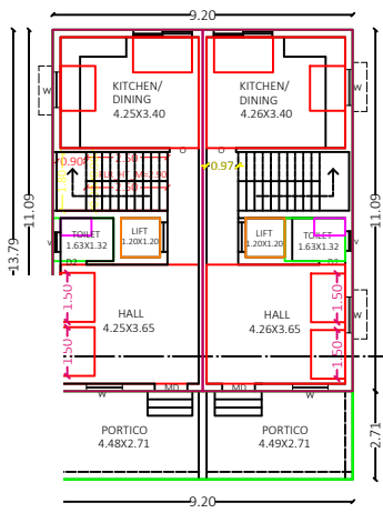
GROUND FLOOR SCALE 1:100
