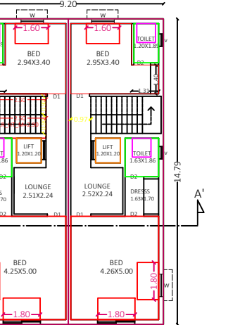
SECOND FLOOR SCALE 1:100
