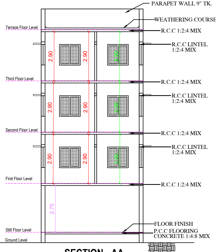
SECTION - AA (PROPOSED)
