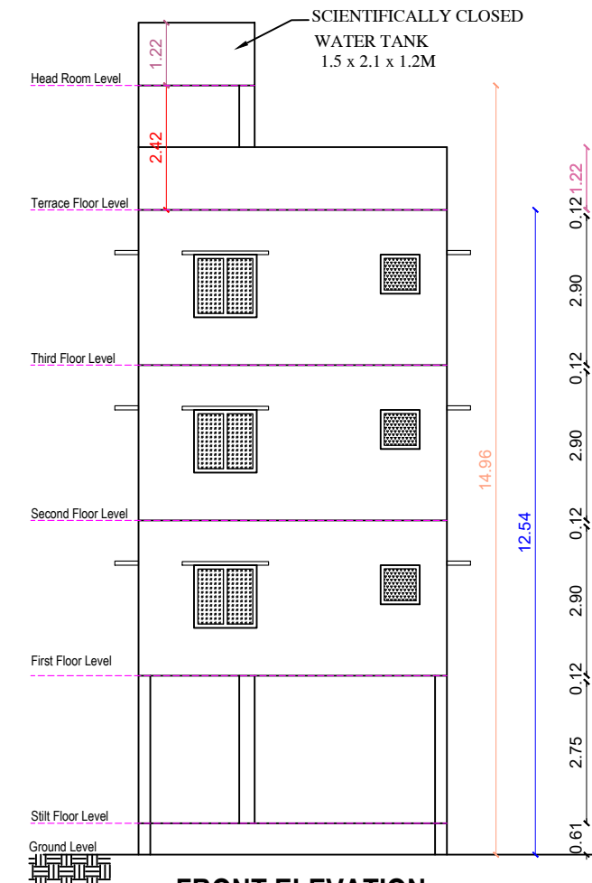
FRONT ELEVATION (PROPOSED)
