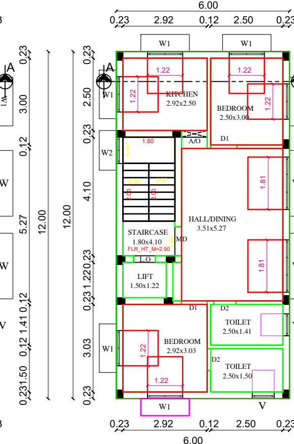
SECOND FLOOR PLAN (PROPOSED)
