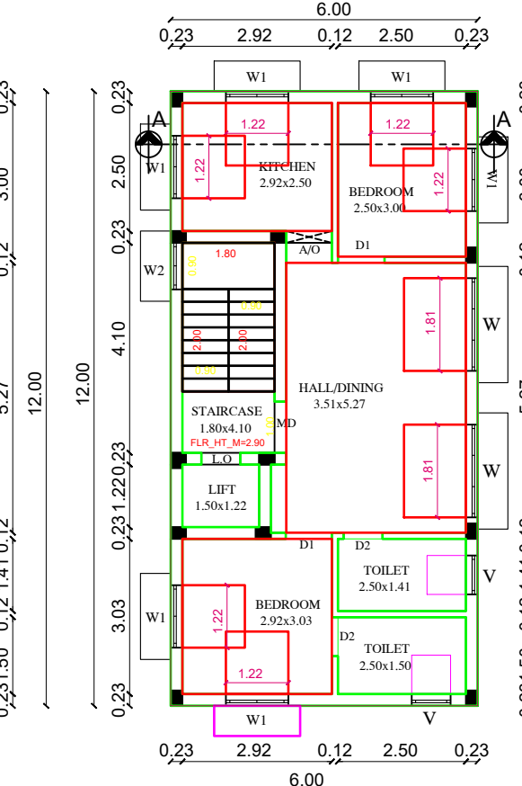
THIRD FLOOR PLAN (PROPOSED)
