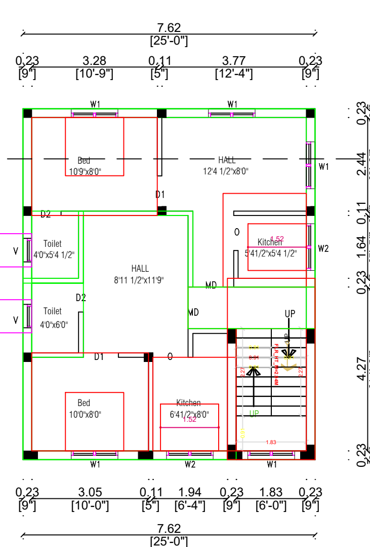
TYPICAL II & III FLOOR
