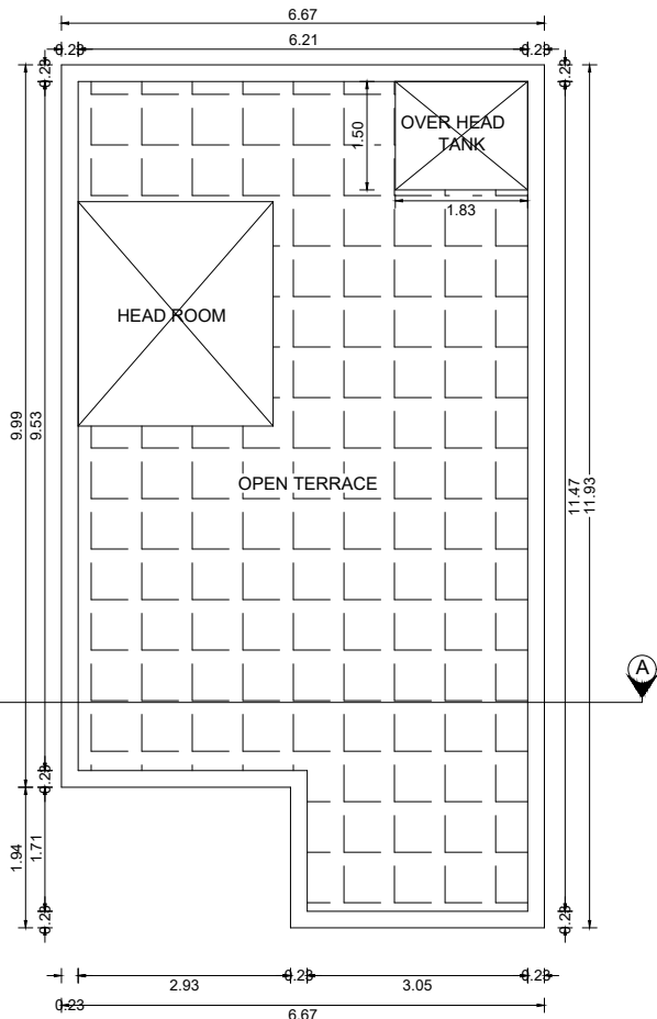
TERRACE FLOOR PLAN (PROPOSED BUILDING)
