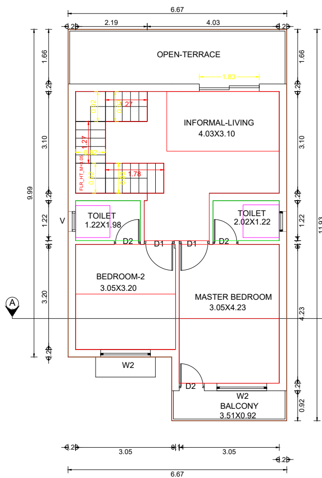
FIRST FLOOR PLAN (PROPOSED BUILDING)
