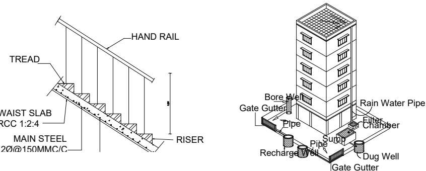
PROPOSED RAIN WATER HARVESTING SYSTEM PROVIDED AS PER TNCDR
