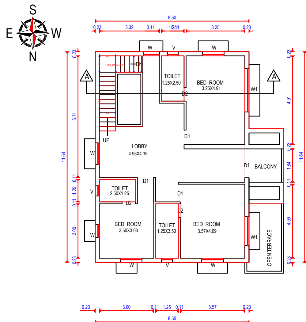
FIRST FLOOR PLAN [PROPOSED]
