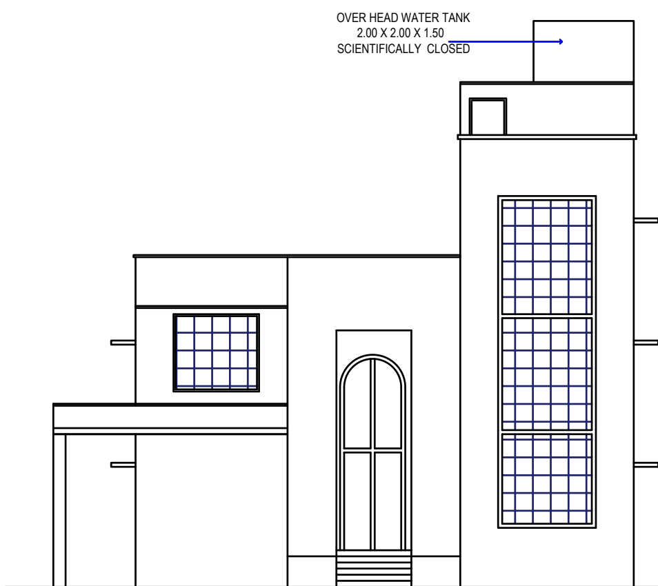
ELEVATION [PROPOSED]
