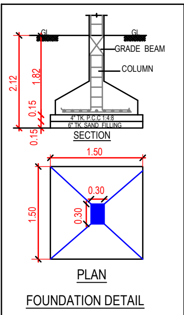
FOUNDATION DETAIL
