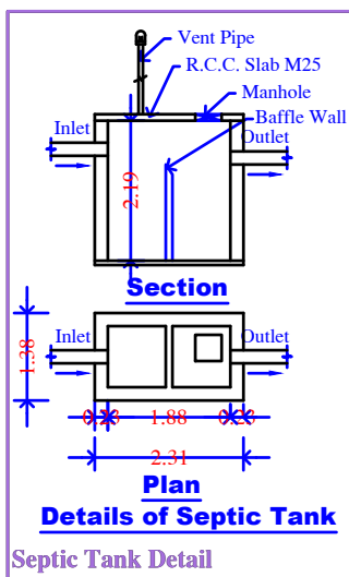
Section Details of Septic Tank
