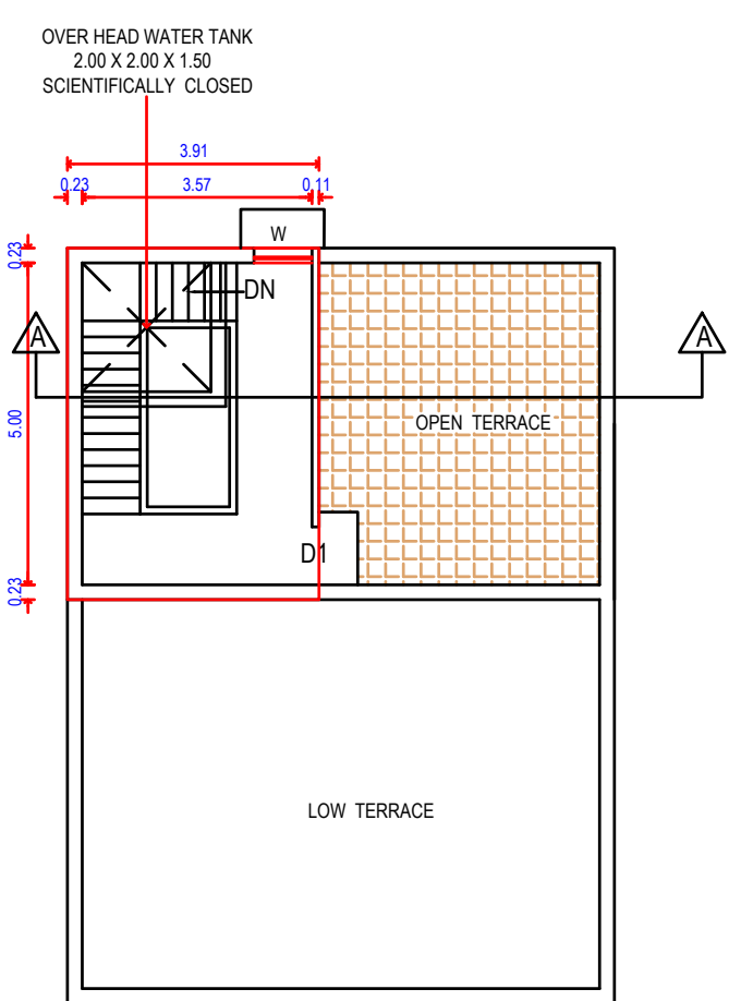
TERACE FLOOR PLAN [PROPOSED]
