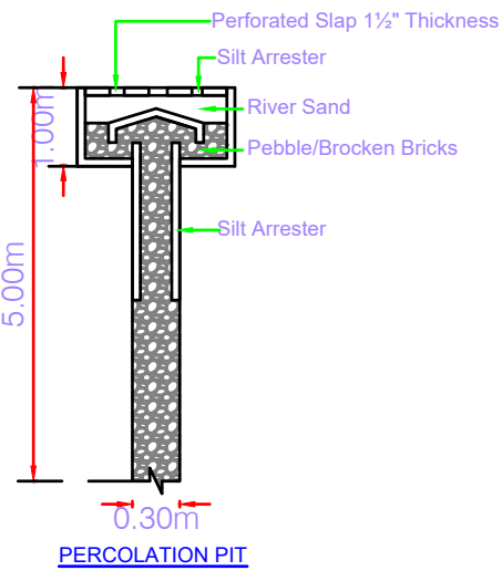
PERCOLATION PIT
