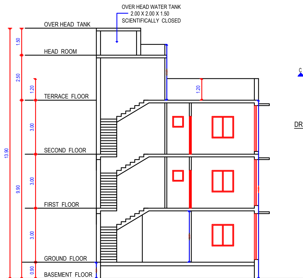
SECTION ON A - A [PROPOSED]
