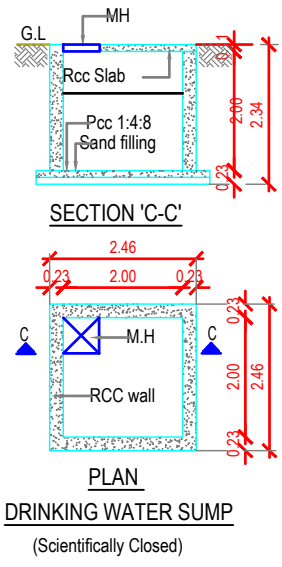
PLAN DRINKING WATER SUMP (Scientifically Closed)
