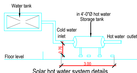
Solar hot water system details
