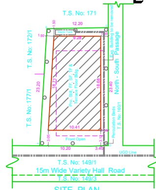
SITE PLAN
