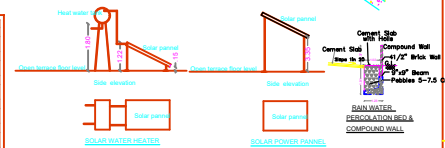
SOLAR WATER HEATER
