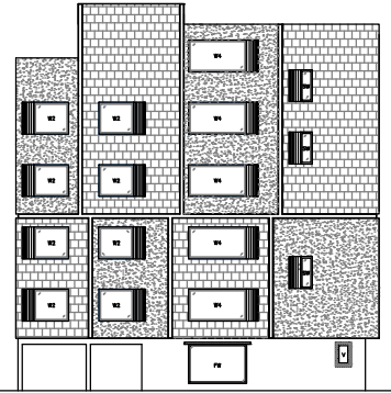
NORTH SIDE ELEVATION
