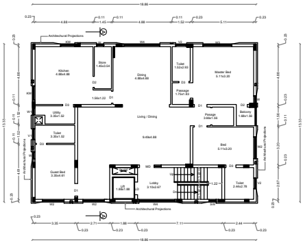
TYPICAL FLOOR PLAN [FIRST, SECOND, THIRD & FOURTH]
