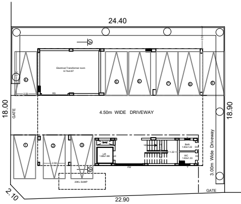
SITE/STILT FLOOR PLAN
