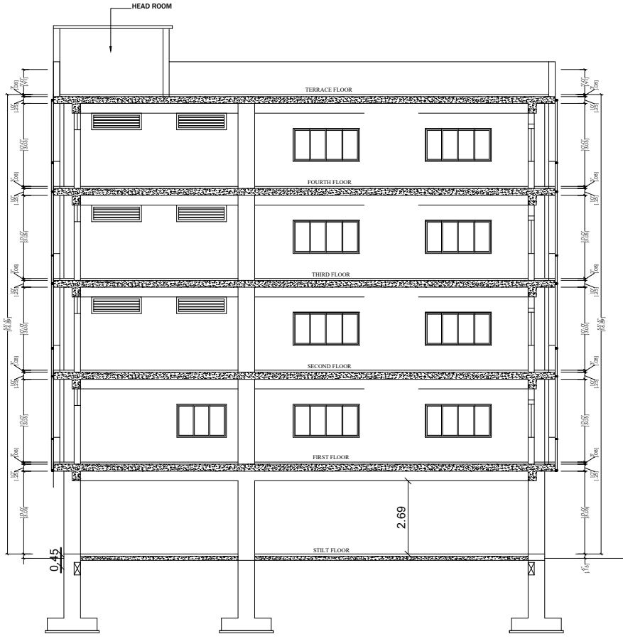
SECTION AT BB
