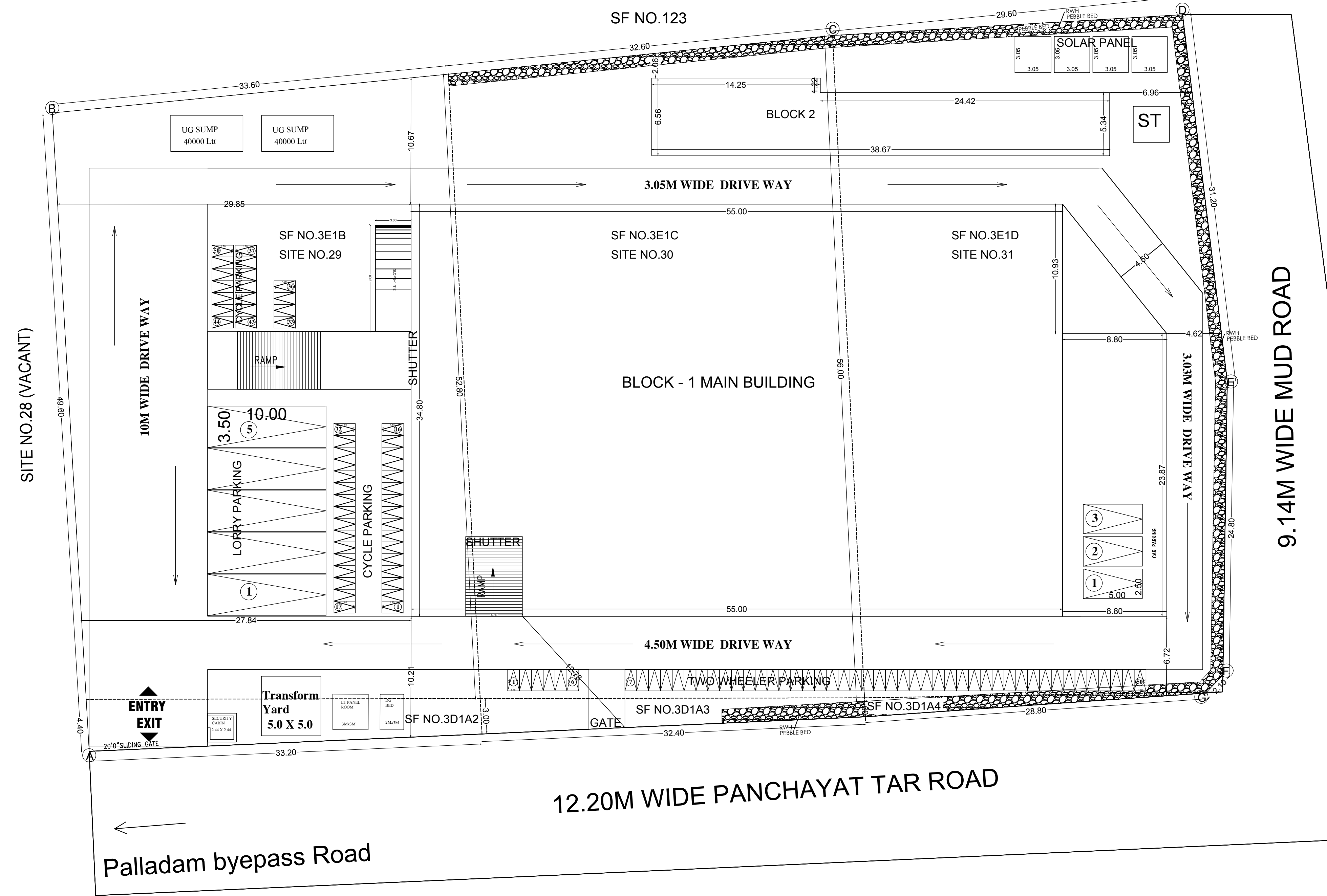
SITE PLAN
