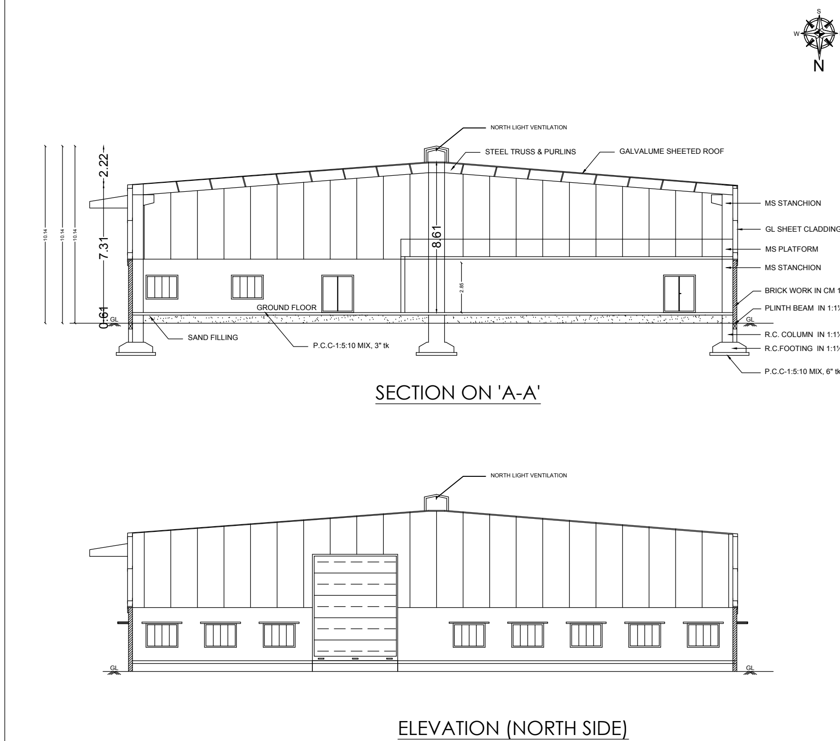
BLOCK-1 G.I. SHEET C ROOF BUILDING
