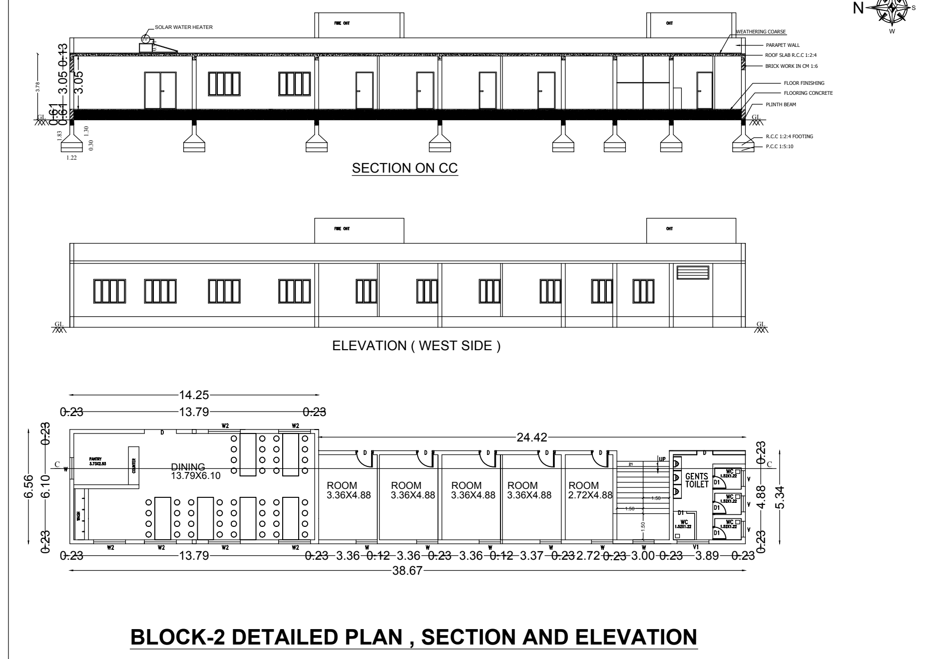
BLOCK-2 R.C.C ROOF BUILDING
