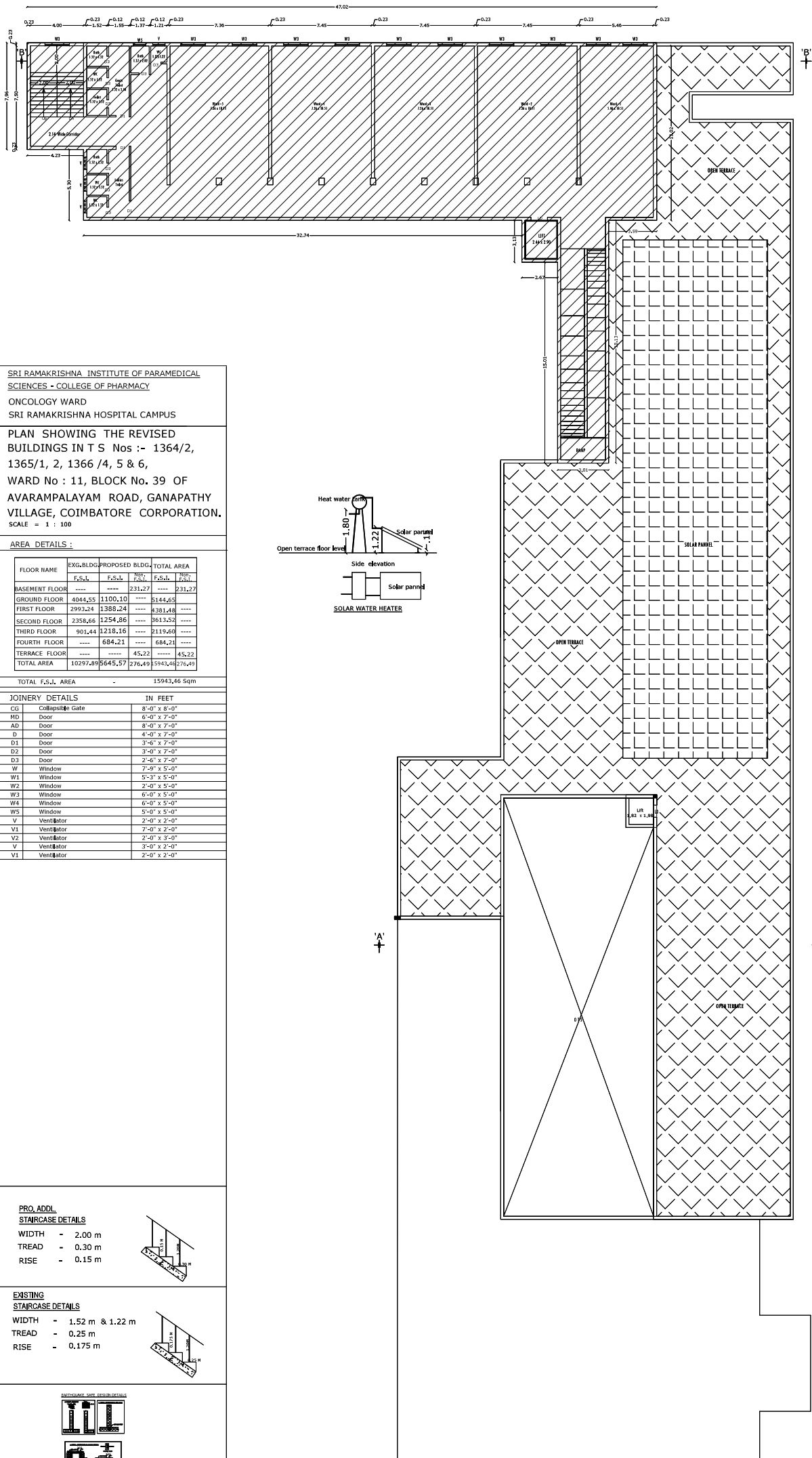
FOURTH FLOOR PLAN
