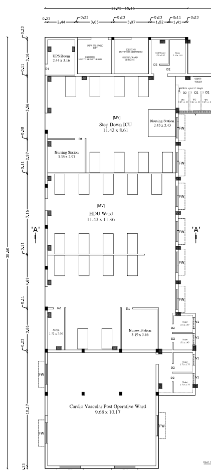
PROPOSED ADDITIONAL SECOND FLOOR
