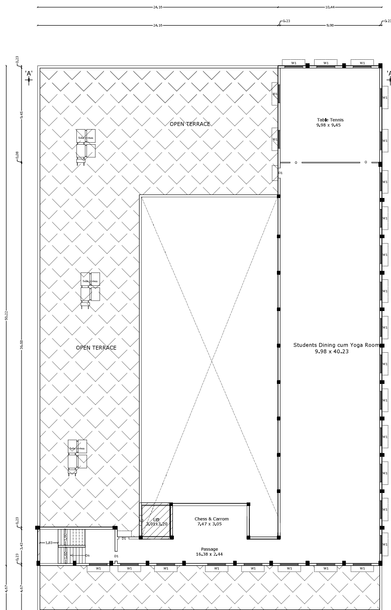
UNDER CONSTRUCTION FOURTH FLOOR PLAN
