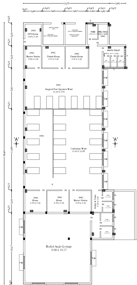
PROPOSED ADDITIONAL FIRST FLOOR
