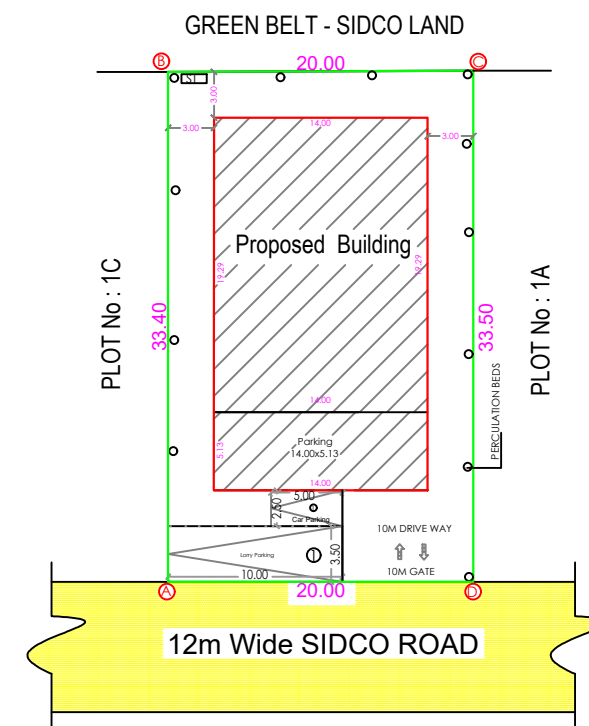
SITE PLAN
