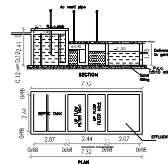
DETAILS OF SEPTIC TANK
