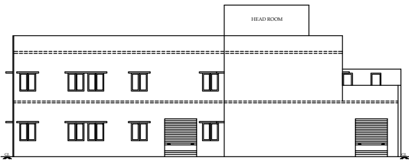
EAST SIDE ELEVATION
