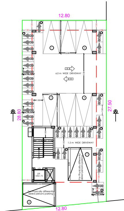
STILT FLOOR PLAN
