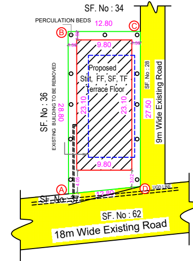
SITE PLAN
