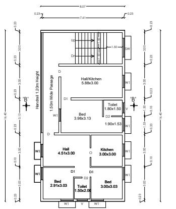
FIRST FLOOR PLAN [STAFF QUARTERS]
