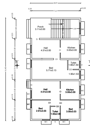
GROUND FLOOR PLAN [STAFF QUARTERS]
