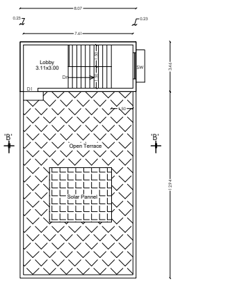
TERRACE FLOOR PLAN [STAFF QUARTERS]
