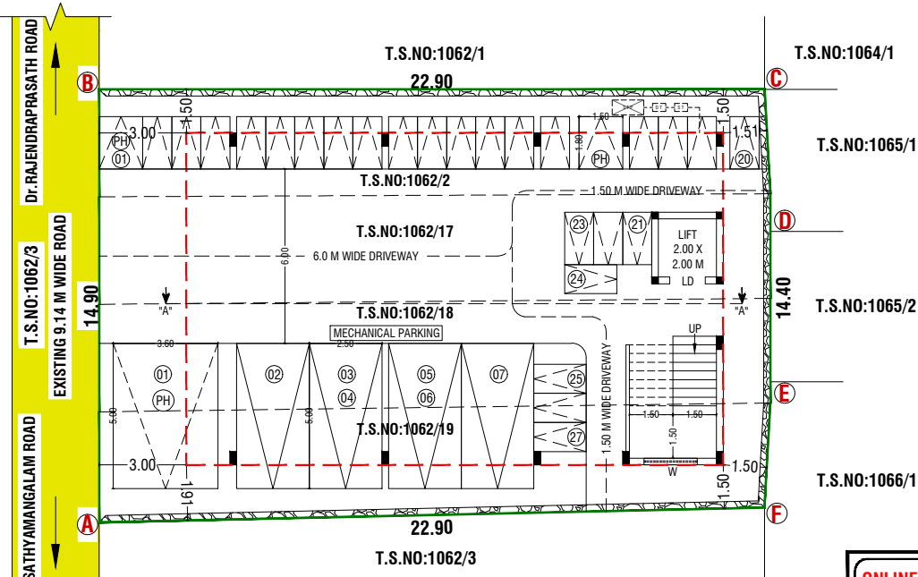
SITE CUM STILT FLOOR PLAN
