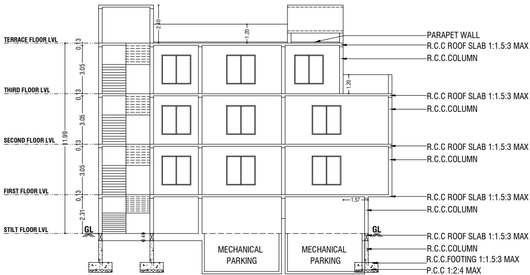
SOUTH SIDE SECTION "AA"
