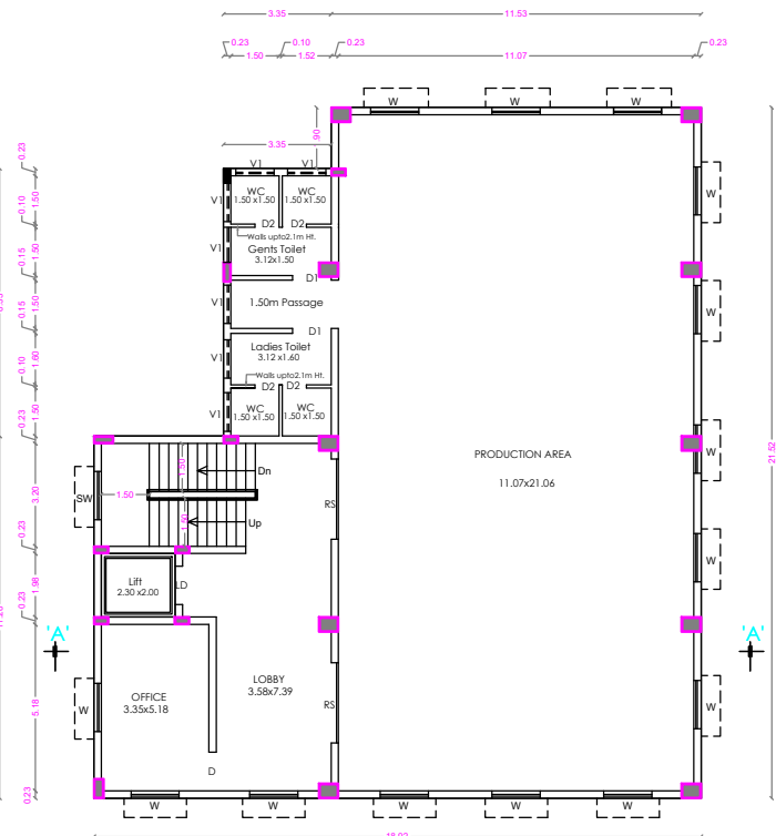
FIRST & SECOND FLOOR PLAN
