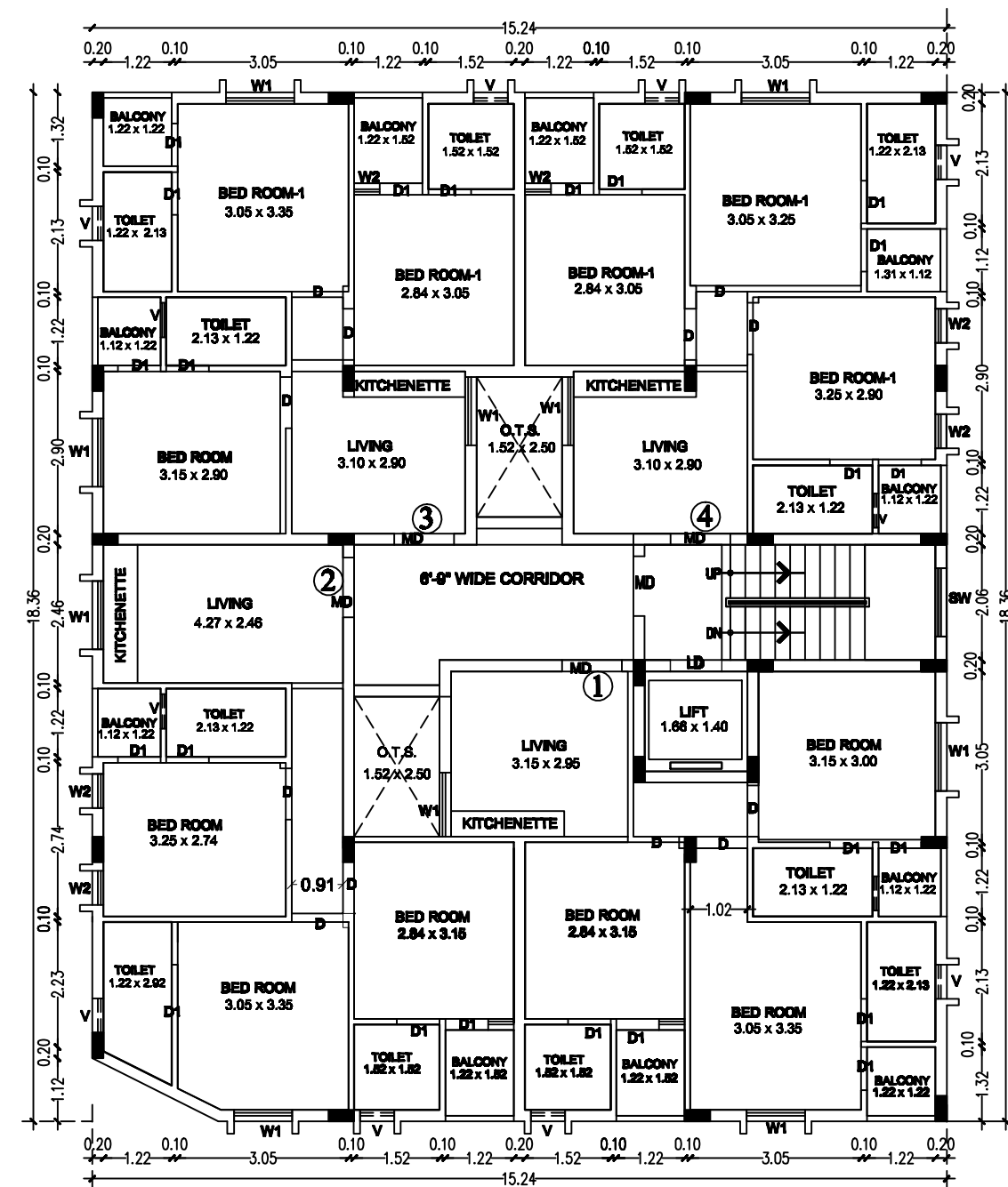
TYPICAL FLOOR PLAN (FIRST,SECOND & THIRD)
