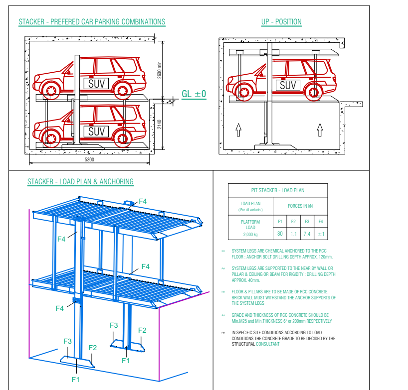
MECHANICAL CAR PARKING DETAILS
