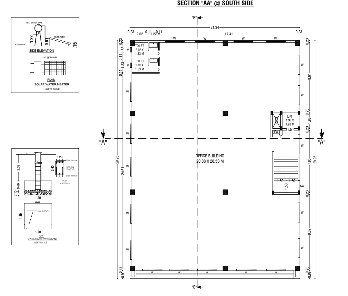
SECTION "AA" @ SOUTH SIDE
