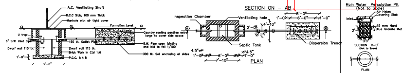
SEPTIC TANK WITH DISPERSION TRENCH ( 250 Gls.)
