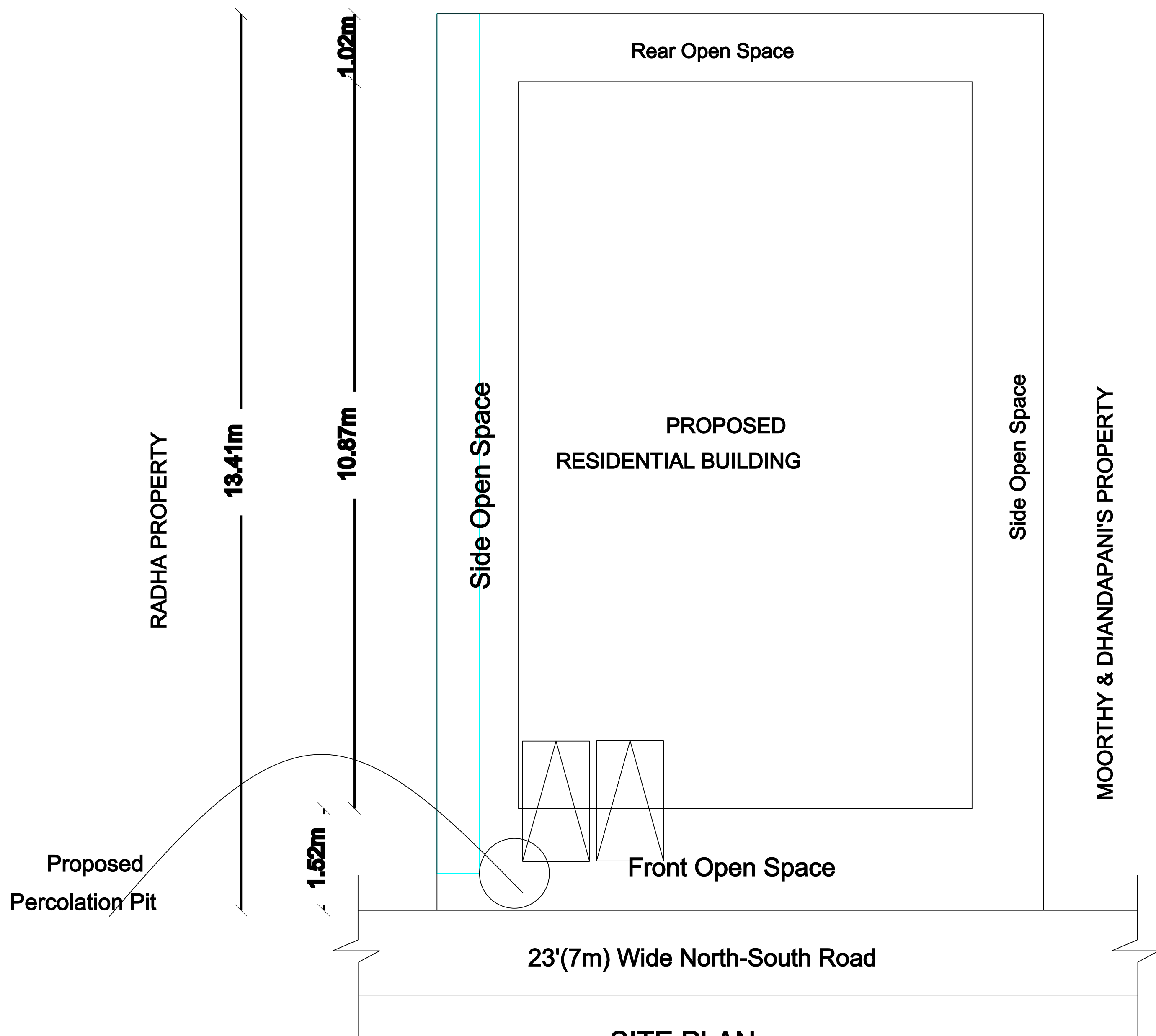
SITE PLAN
