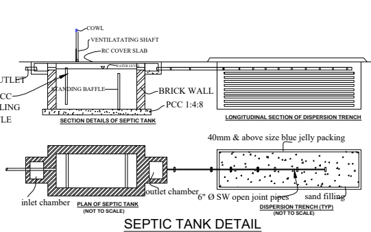
SEPTIC TANK DETAIL
