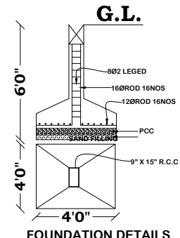
FOUNDATION DETAILS
