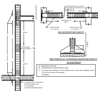
SEISMIC REINFORCEMENT DETAILS
