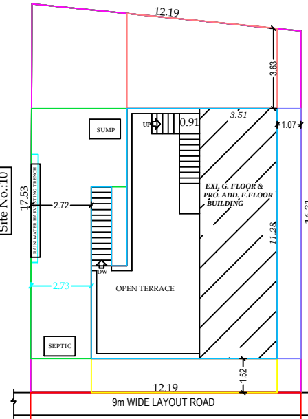
SITE PLAN
