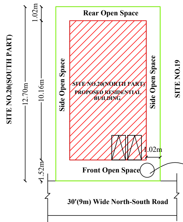
SITE PLAN
