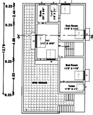
PRO.FIRST FLOOR PLAN
